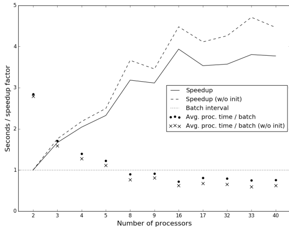
Figure 9: Dimension: d = 2
