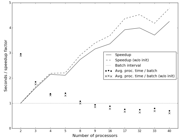
Figure 8: Dimension: d = 100
