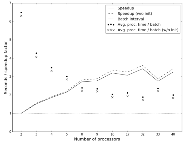
Figure 10: Dimension: d = 100
